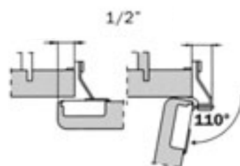
CHARNIÈRE "FACE FRAME" 45mm C.C. / GOUJONS 8mm FACE FRAME HINGE 45mm C.C. / 8mm DOWELS
